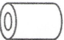
#18 Installing cup O.D.: 2" I.O.: 1-3/4" Length: 2-5/16"
