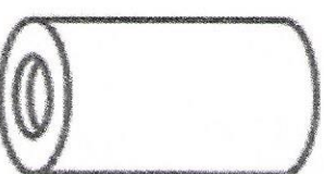
#21 Install cup O.D.: 2" I.O.: 1-3/4" Length: 3"
