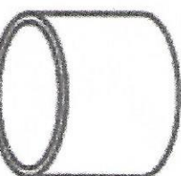
#14 Receiving tube O.D.: 2-3/4" I.O.: 1-7/16" Length: 2-1/4"
